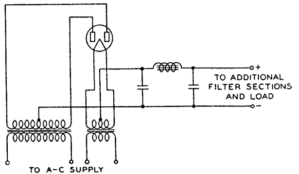
CONDENSER INPUT FILTER CIRCUIT B
